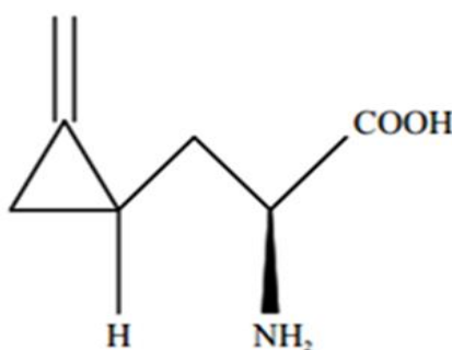
Figure 5 Structure of hypoglycin A [17, 18]
